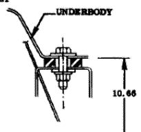
# 5 A BODY MOUNTING CONVERTIBLE ONLY
