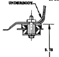
② #3 A BODY MOUNTING SPORT COUPE ONLY
