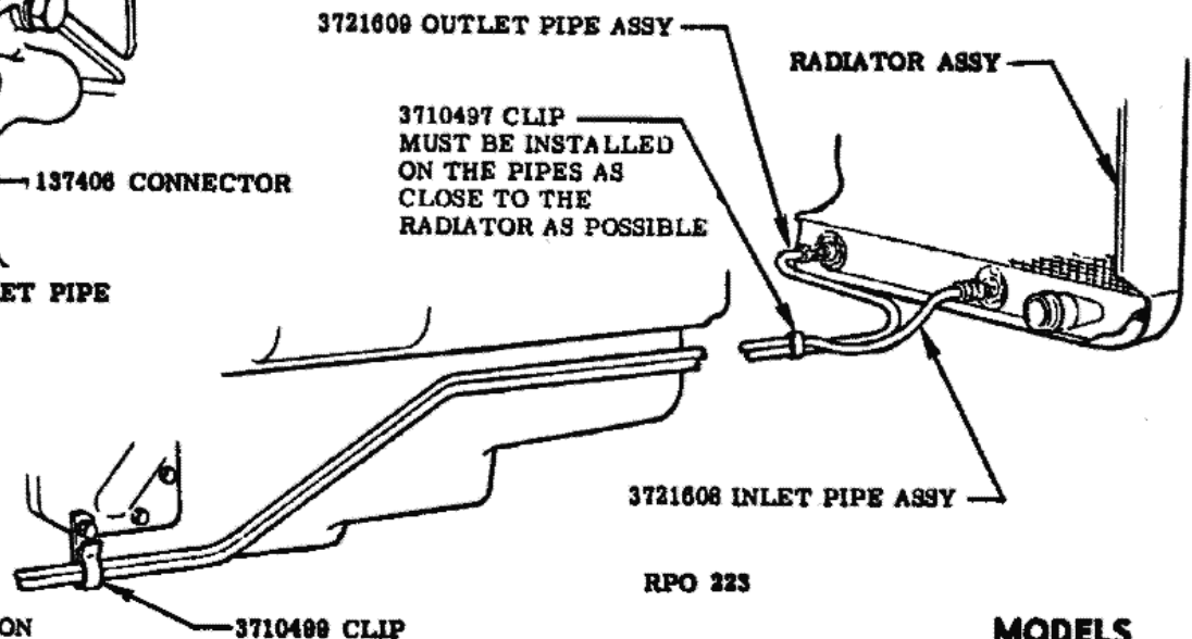
VIEW A
