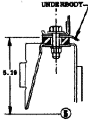
71 BODY MOUNTING CONVERTIBLE ONLY
