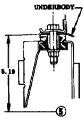
# 1 BODY MOUNTING ALL EXCEPT CONV
