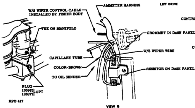
LEFT DRIVE
