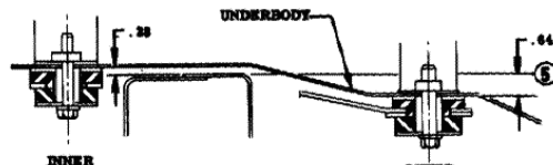
83 BODY MOUNTING ALL EXCEPT CONV
