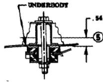
# 2 OUTER BODY MOUNTING ALL EXCEPT CONV
