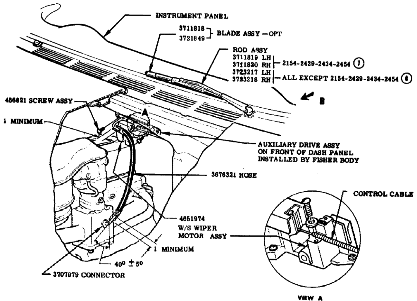
SHOWING CONNECTION OF CONTROL CABLE &amp; W/S WIPER MOTOR
