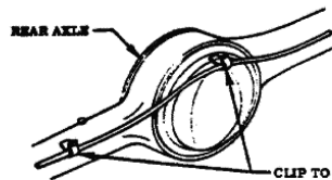
VIEW F
