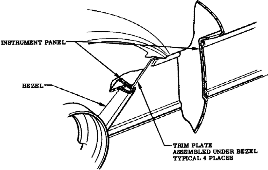
VIEW B
