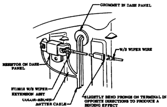
RIGHT DRIVE
