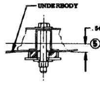
#2 OUTER BODY MOUNTING CONVERTIBLE ONLY
