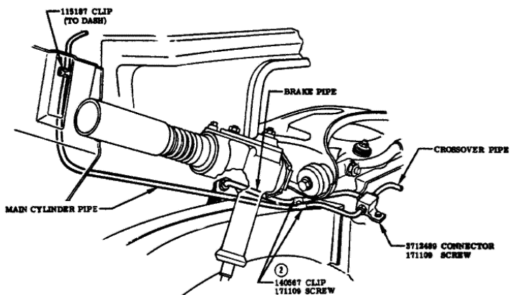
VIEW C
