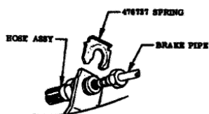
VIEW 8
