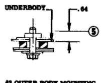
#3 OUTER BODY MOUNTING CONVERTIBLE ONLY
