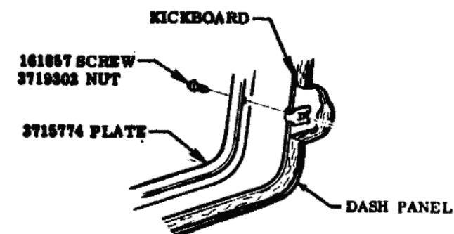
VIEW A
