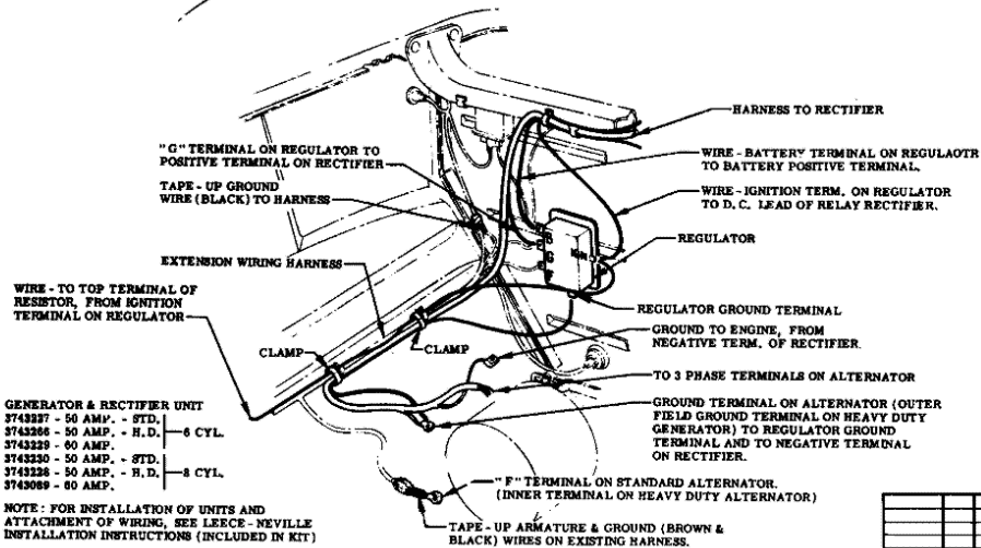
VIEW A (8 CYLINDER)
