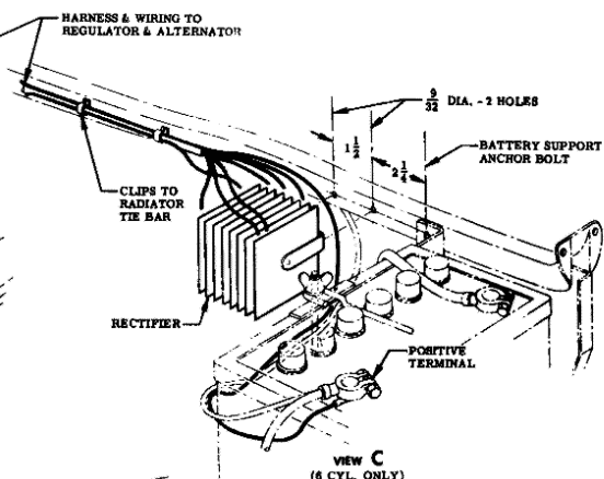
VIEW C (6 CYL. ONLY)
