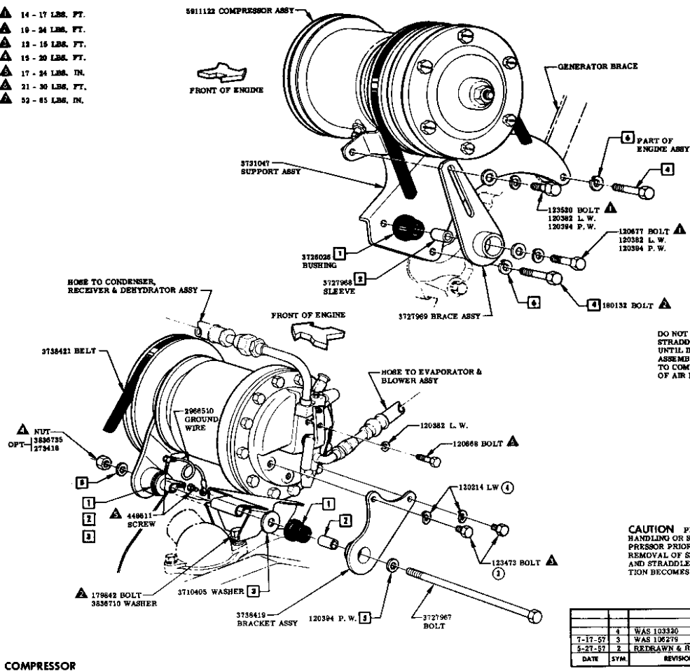
COMPRESSOR
