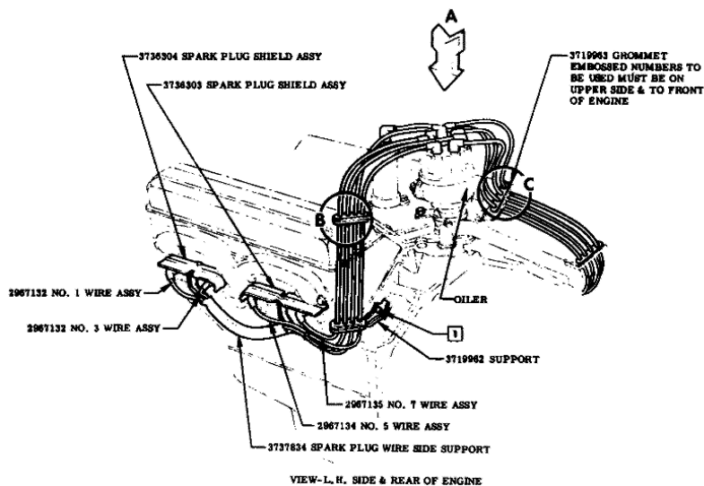
VIEW-L, H. SIDE & REAR OF ENGINE
