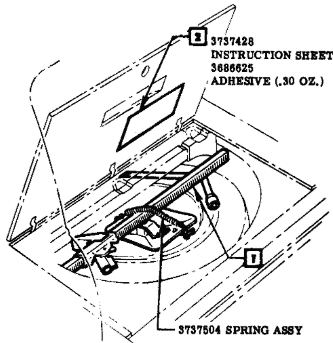
STATION WAGON (EXCEPT 9 PASS.) & SEDAN DELIVERY
