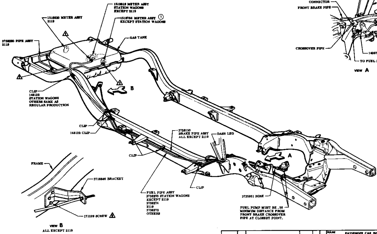
FUEL & BRAKE LINE
