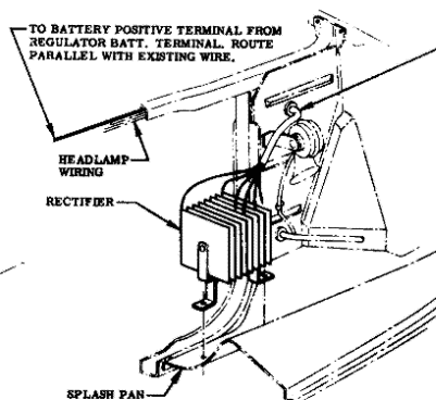
VIEW D (8 CYL. ONLY)
