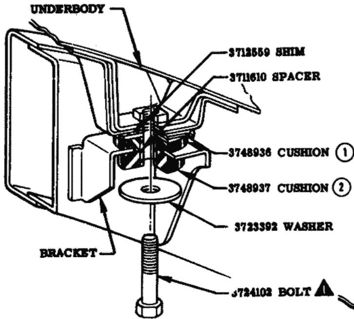
VIEW A 9 PASSENGER STATION WAGON
