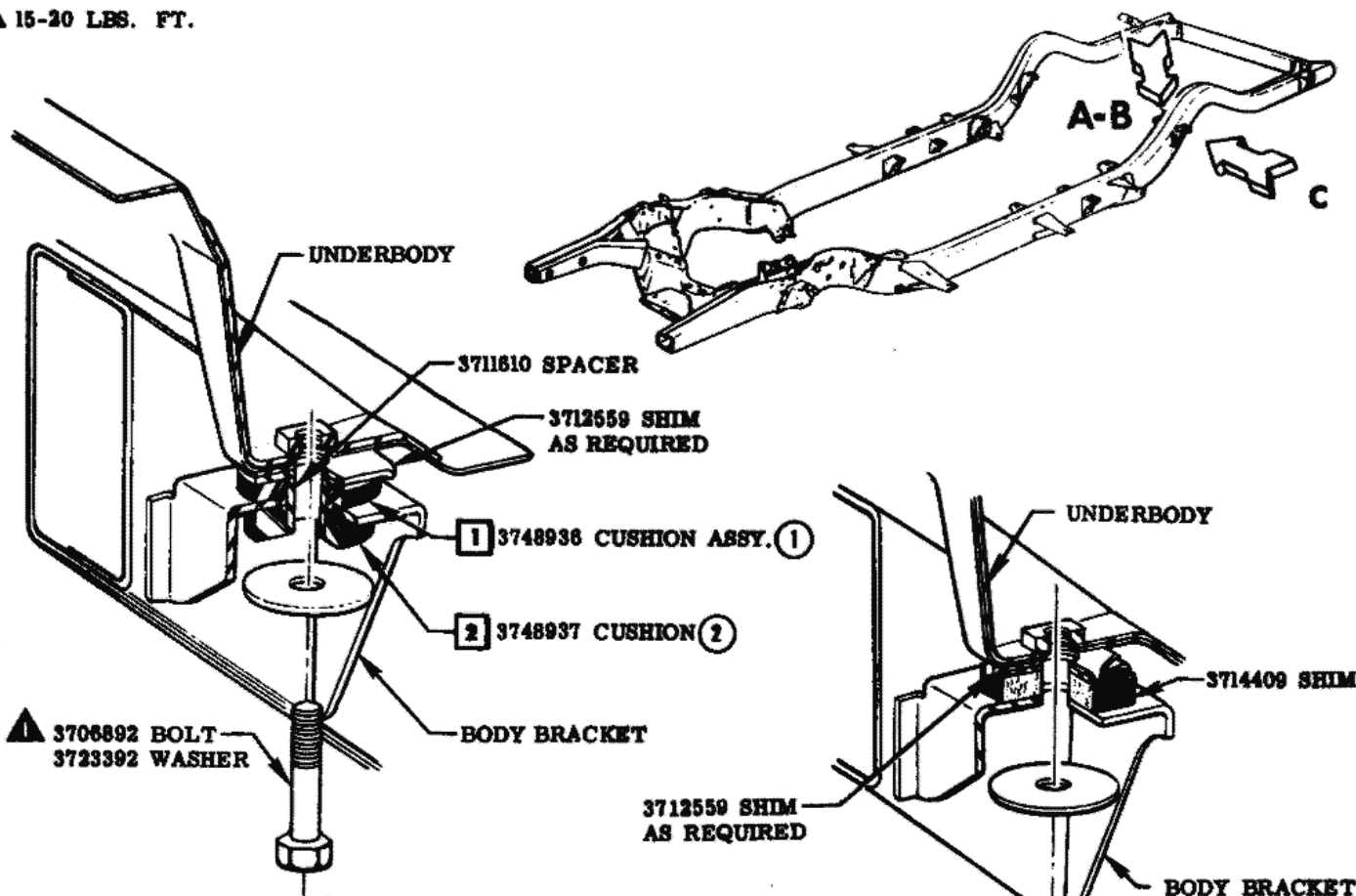
VIEW A ALL EXCEPT CONVERTIBLE & 9 PASSENGER STATION WAGON
