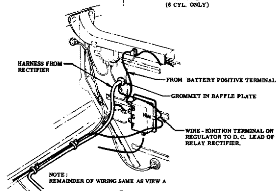
VIEW B (6 CYLINDER)
