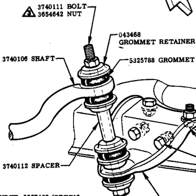
VIEW B
