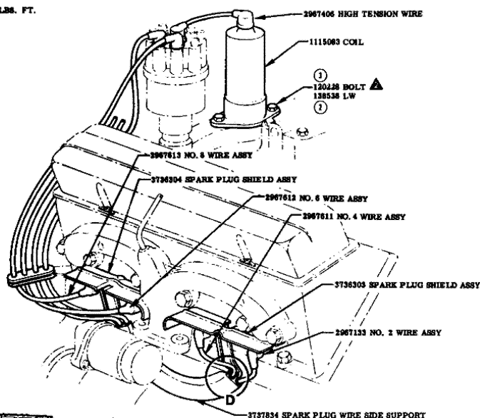
VIEW-R, H. SIDE OF ENGINE
