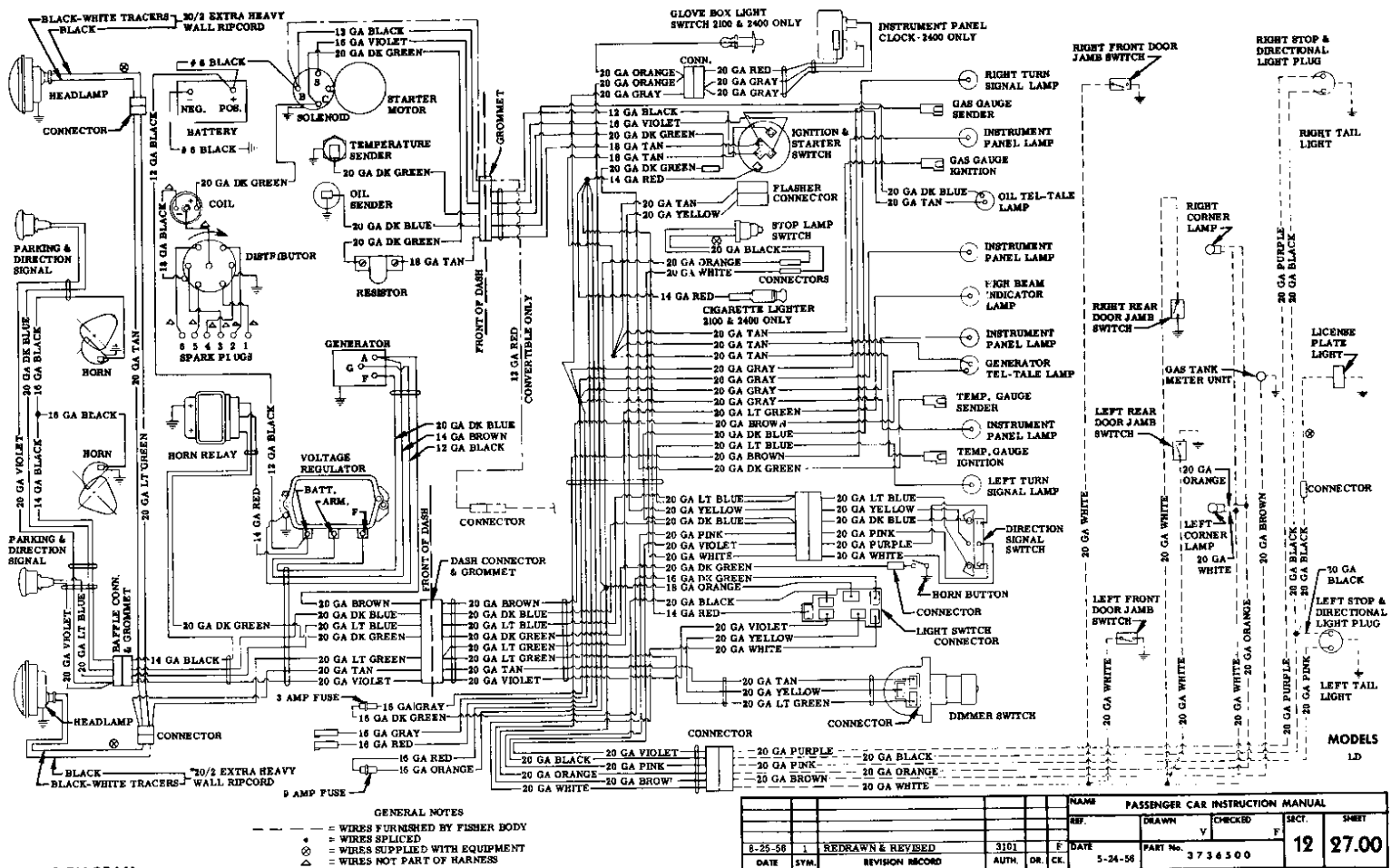
WIRING DIAGRAM
