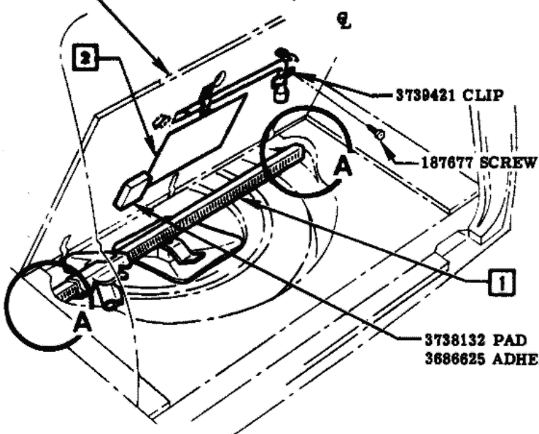
9 PASSENGER STATION WAGON
