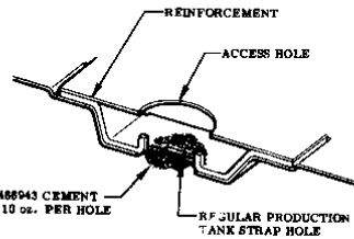
VIEW D
