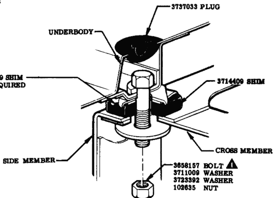
VIEW B CONVERTIBLE
