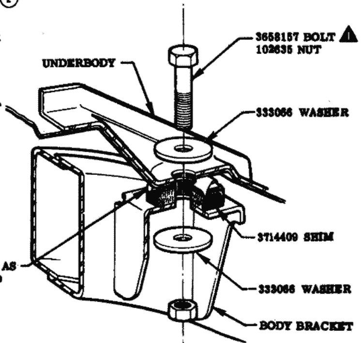
VIEW B CONVERTIBLE
