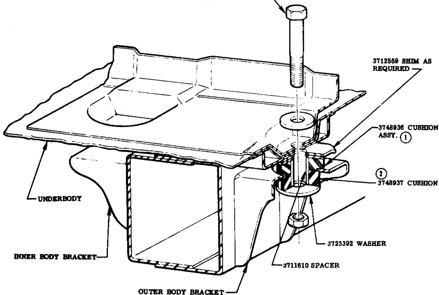
VIEW A
