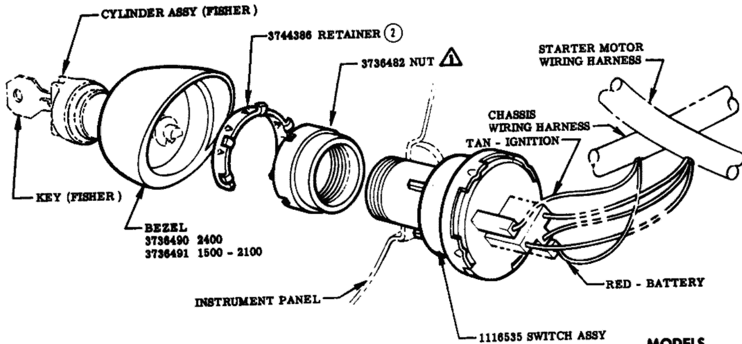
LEFT DRIVE
