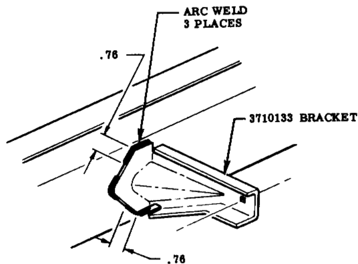
VIEW A
