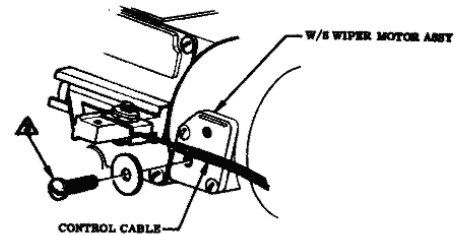
VIEW A SHOWING CONNECTION OF CONTROL CABLE & W/S WIPER MOTOR
