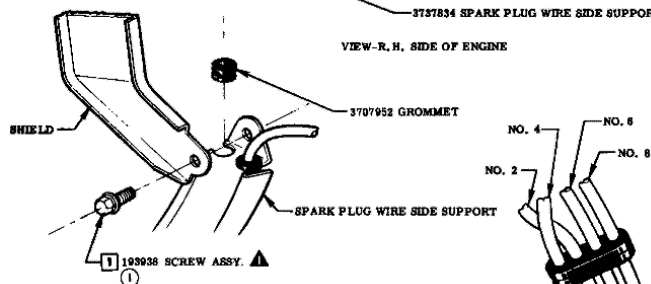
VIEW D
