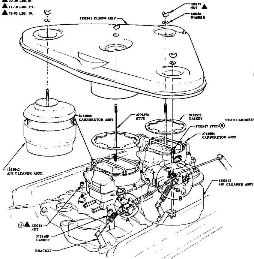
CARBURETOR, AIR CLEANER & LINKAGE
