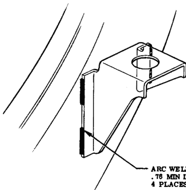
VIEW A
