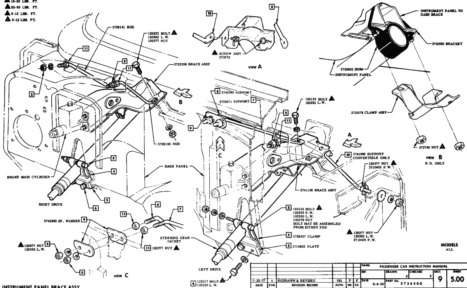
INSTRUMENT PANEL BRACE ASSY.
