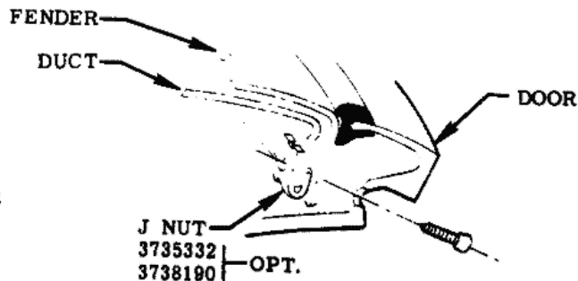
VIEW B
