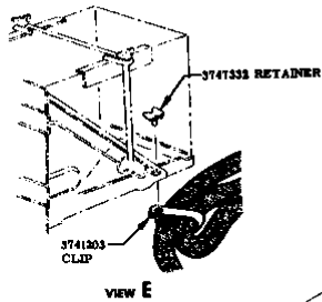
V-8 HOSE ATTACHMENT FOR RECIRCULATING HEATER
