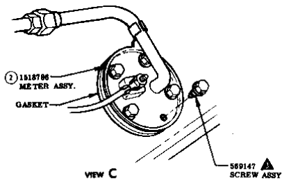
VIEW C
