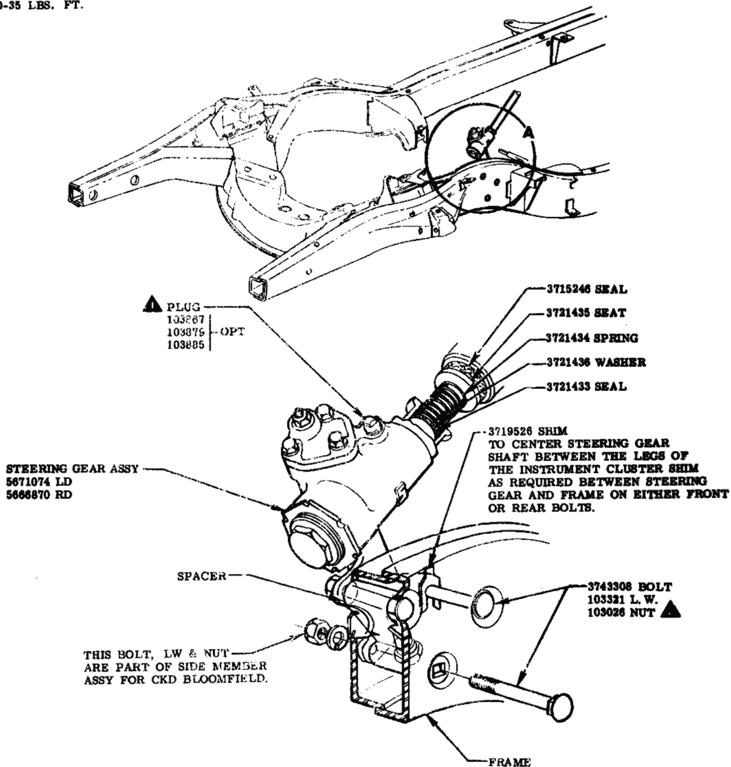
VIEW A
