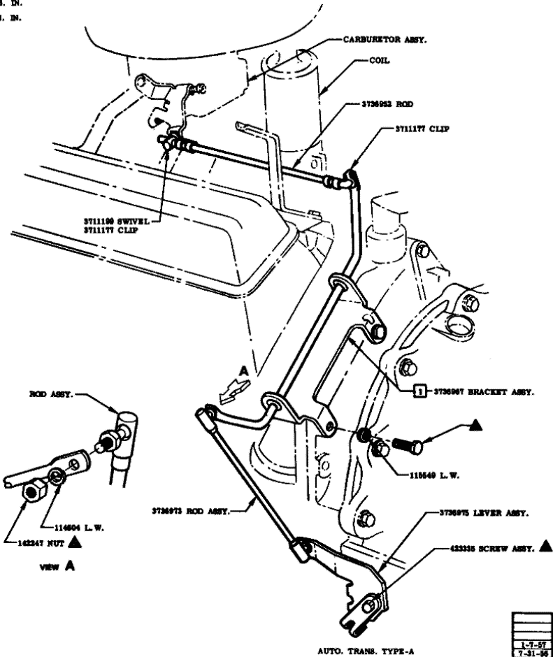
CARBURETOR TO TRANSMISSION LINKAGE
