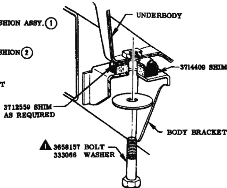
VIEW B CONVERTIBLE
